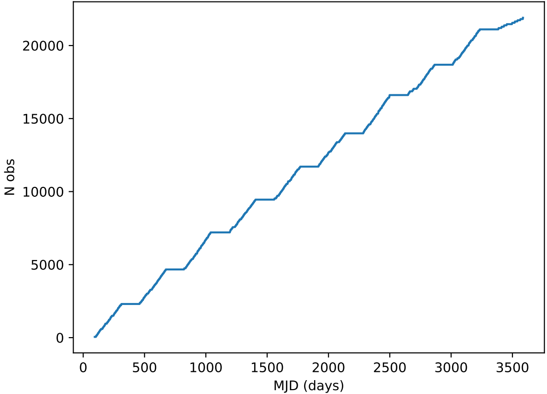
too_elab_heavy_r128_d3_griz_v3.4_10yrs all bands: DD:ECDFS Cumulative NVisits
