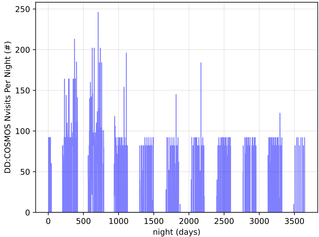
too_elab_heavy_r128_d3_griz_v3.4_10yrs all bands: DD: COSMOS Nvisits Per Night
