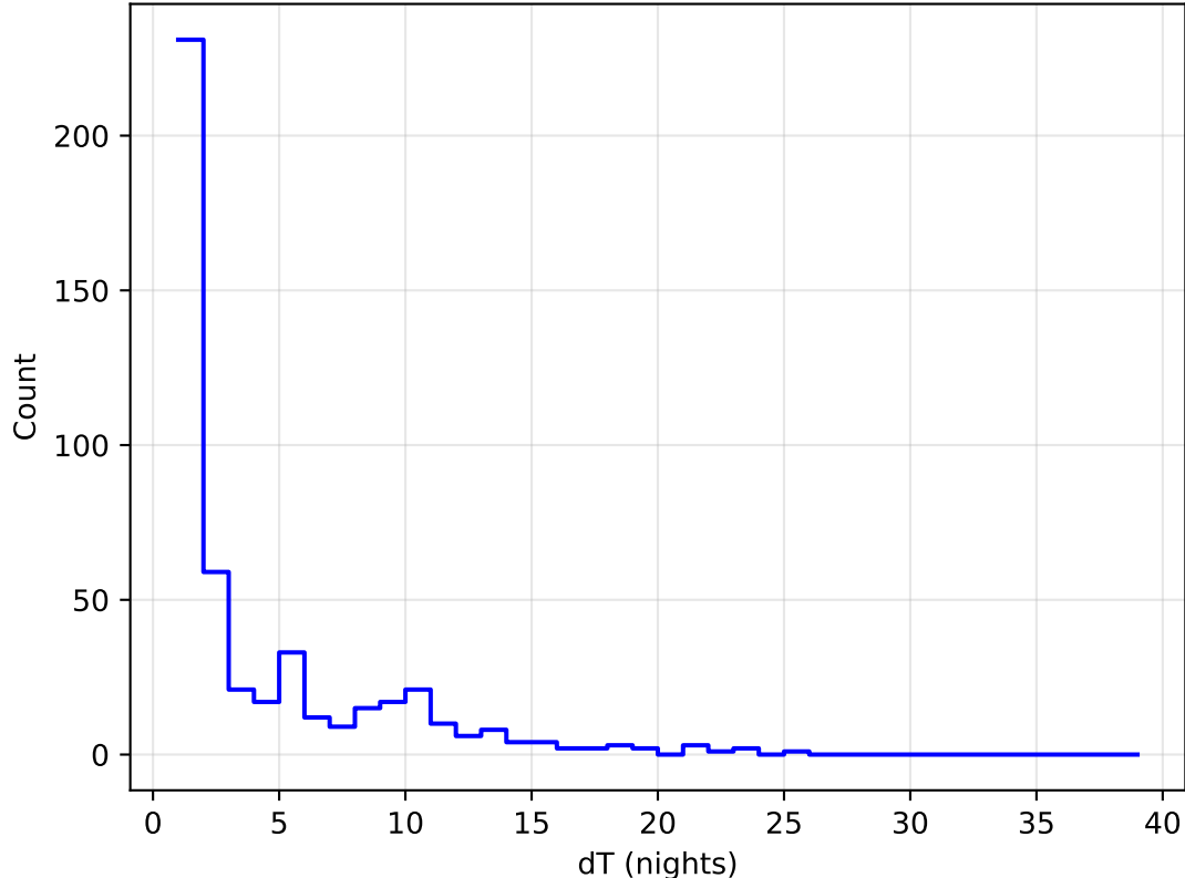
too_elab_heavy_r128_d3_griz_v3.4_10yrs all bands: DD: COSMOS Delta Nights Histogram
