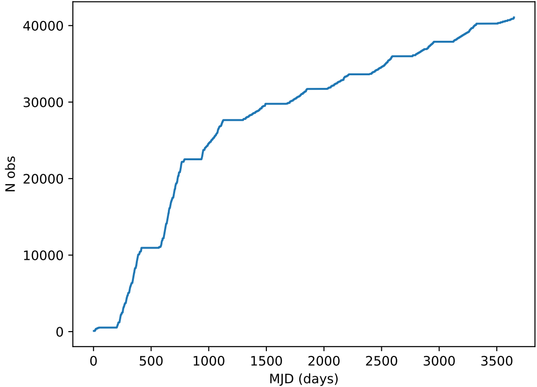
too_elab_heavy_r128_d3_griz_v3.4_10yrs all bands: DD: COSMOS Cumulative NVisits
