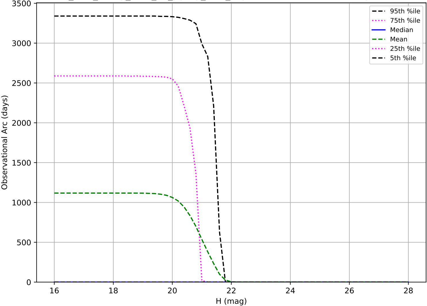
too_elab_heavy_r128_d2_ugrizy_v3.4_10yrs: Observational Arc Length Vatira
