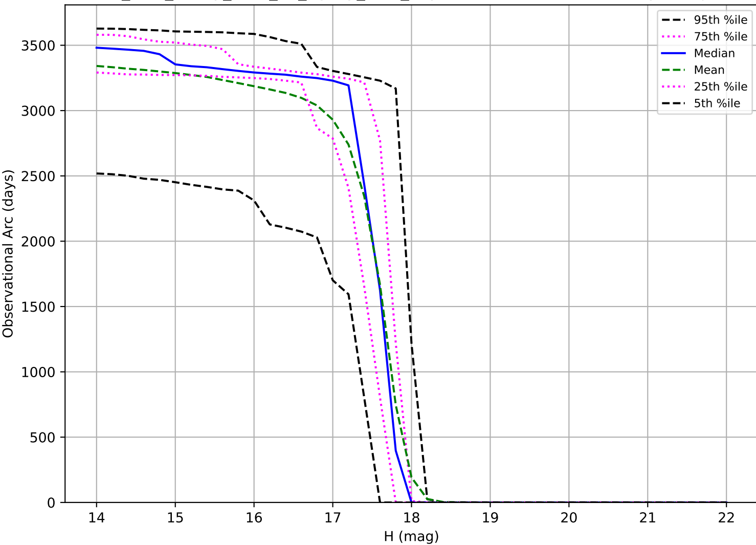
too_elab_heavy_r128_d2_ugrizy_v3.4_10yrs: Observational Arc Length Trojan
