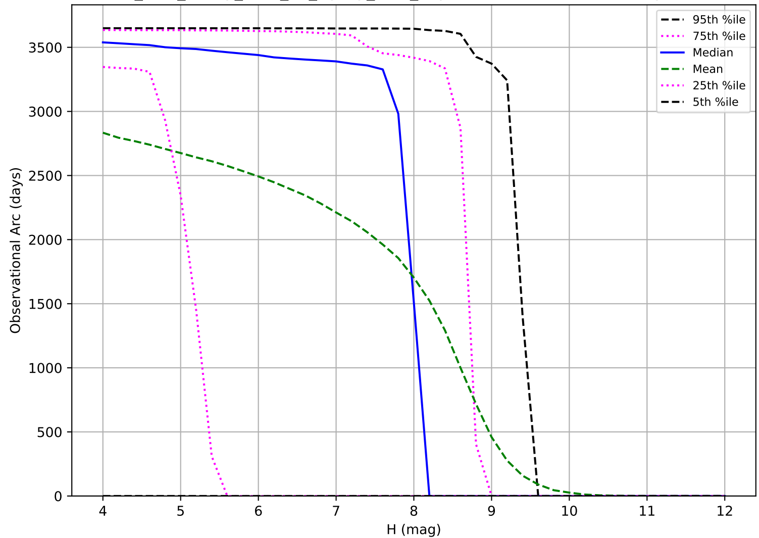
too_elab_heavy_r128_d2_ugrizy_v3.4_10yrs: Observational Arc Length TNO
