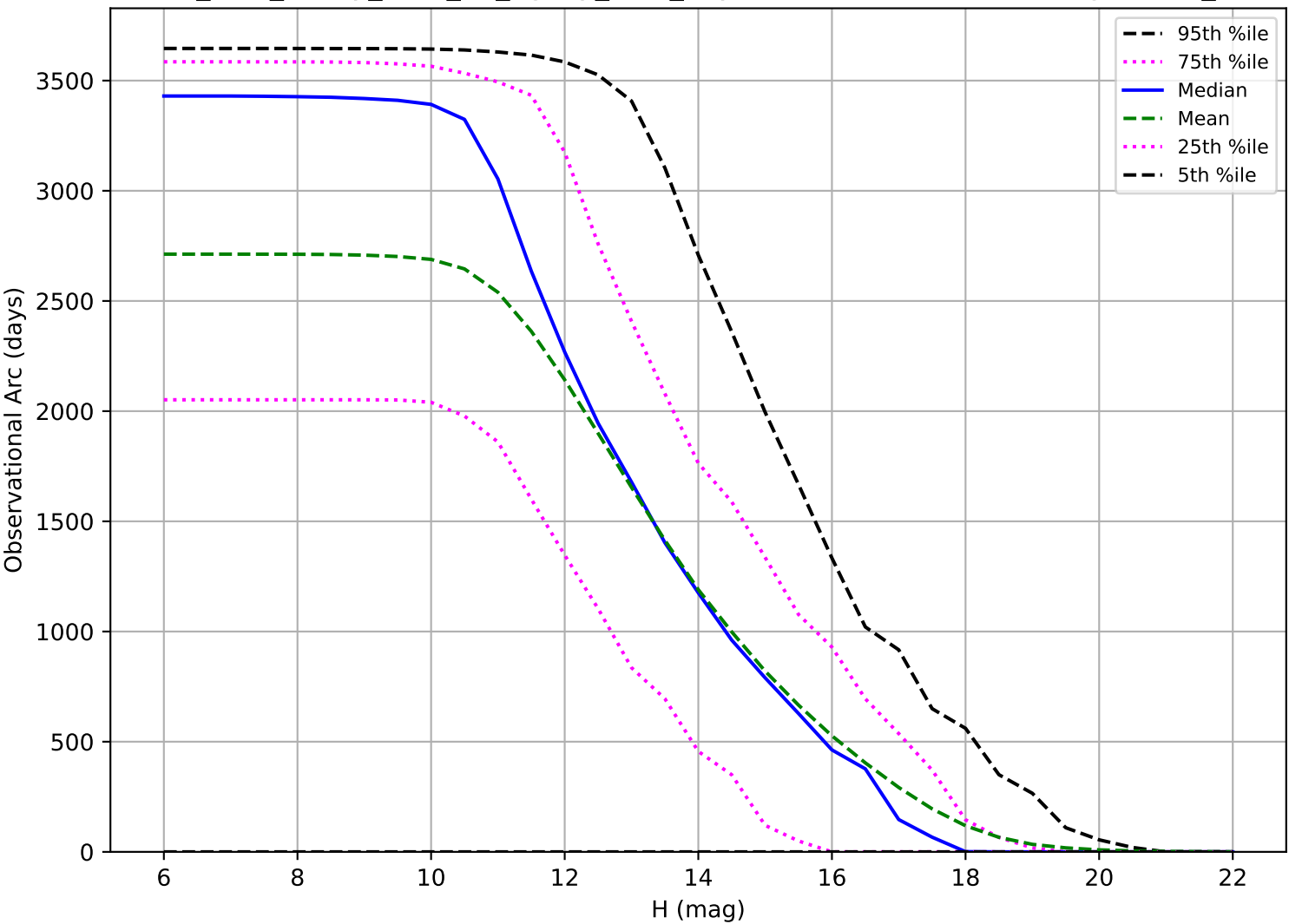
too_elab_heavy_r128_d2_ugrizy_v3.4_10yrs: Observational Arc Length OCC_r5
