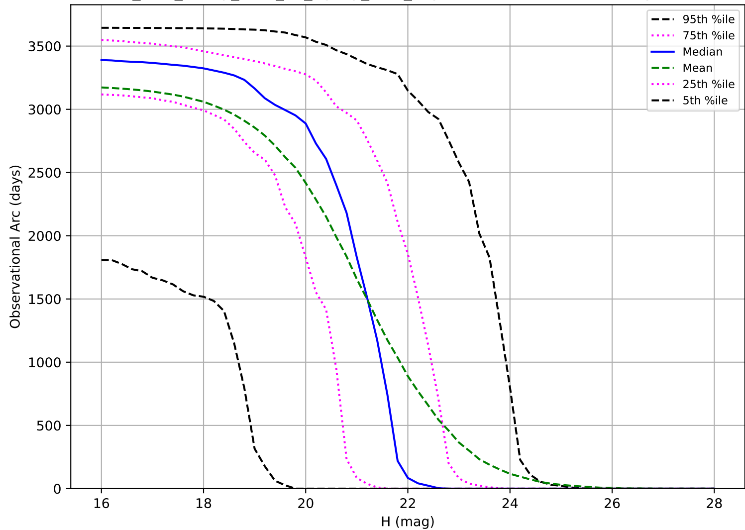
too_elab_heavy_r128_d2_ugrizy_v3.4_10yrs: Observational Arc Length NEO
