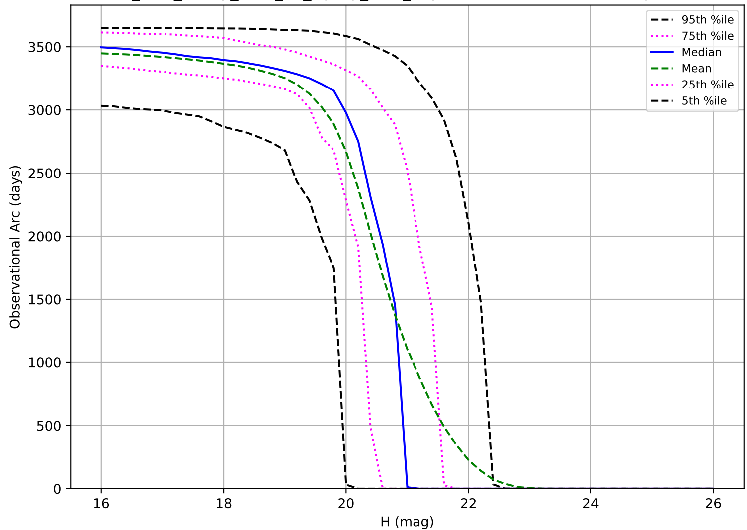
too_elab_heavy_r128_d2_ugrizy_v3.4_10yrs: Observational Arc Length MBA
