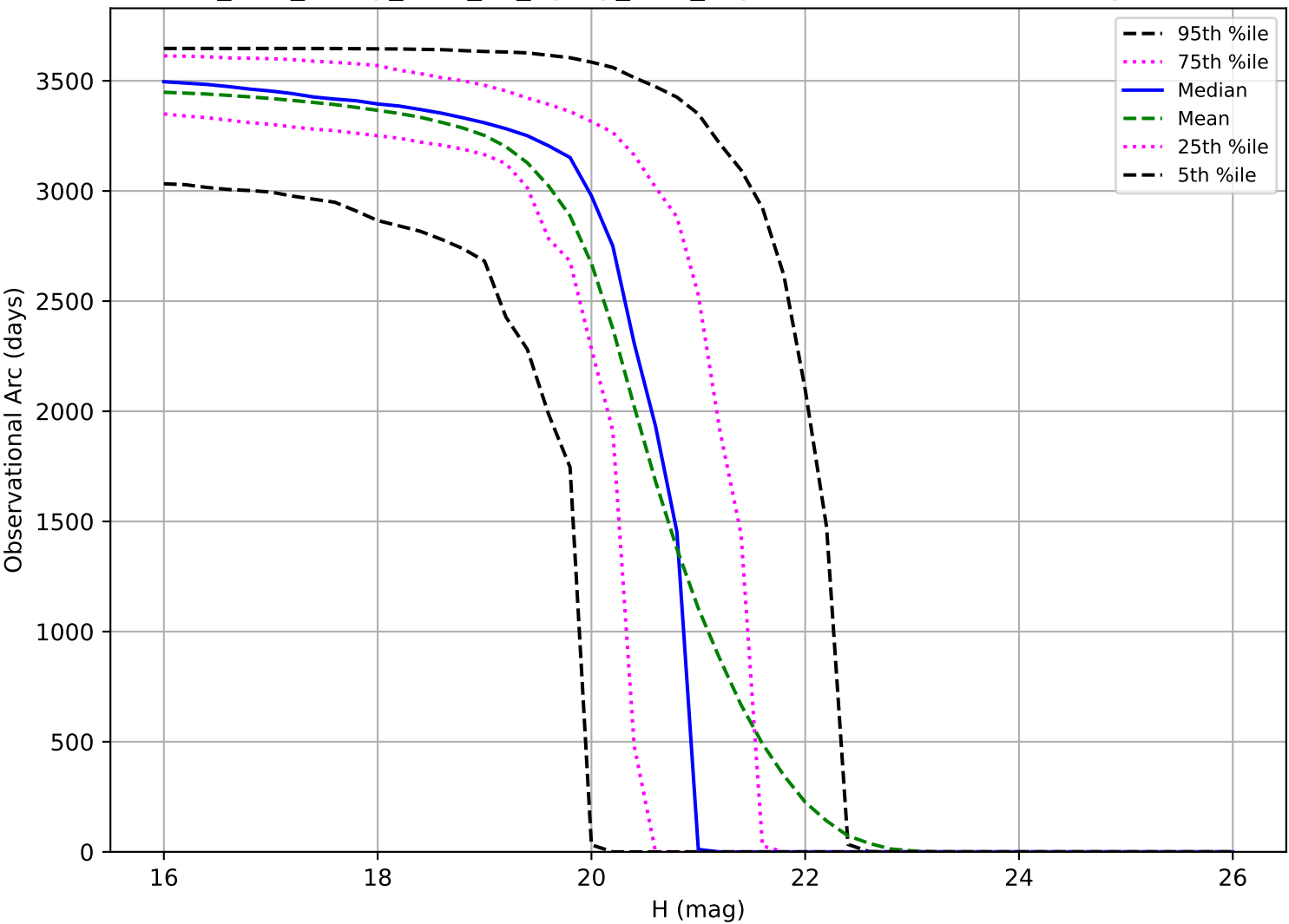
too_elab_heavy_r128_d2_ugrizy_v3.4_10yrs: Observational Arc Length MBA
