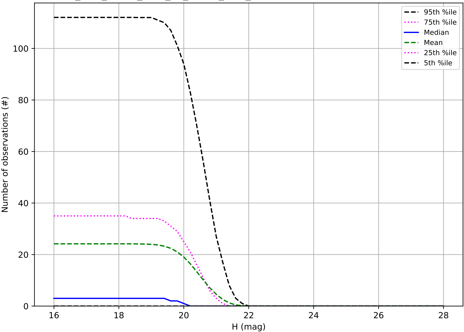
too_elab_heavy_r128_d2_ugrizy_v3.4_10yrs: Number of observations Vatira
