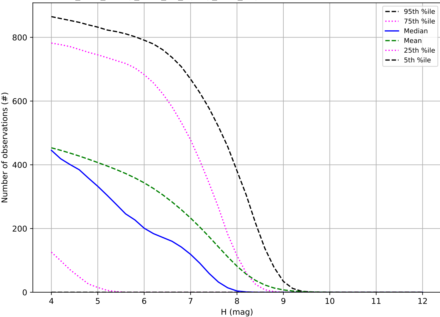
too_elab_heavy_r128_d2_ugrizy_v3.4_10yrs: Number of observations TNO
