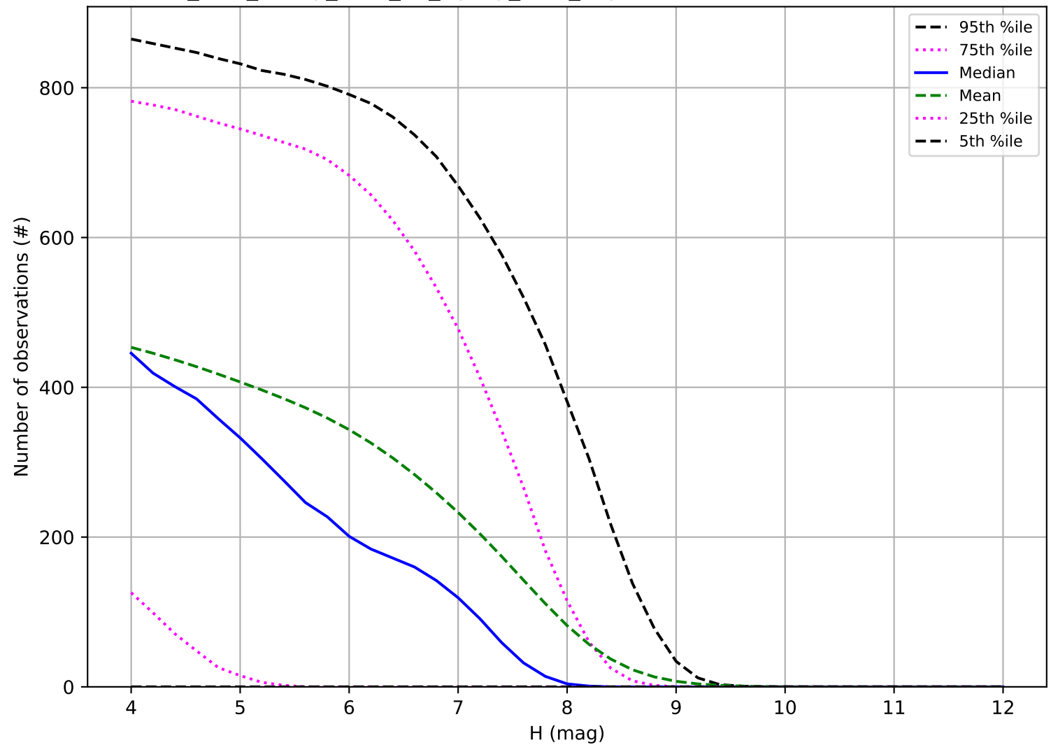
too_elab_heavy_r128_d2_ugrizy_v3.4_10yrs: Number of observations TNO
