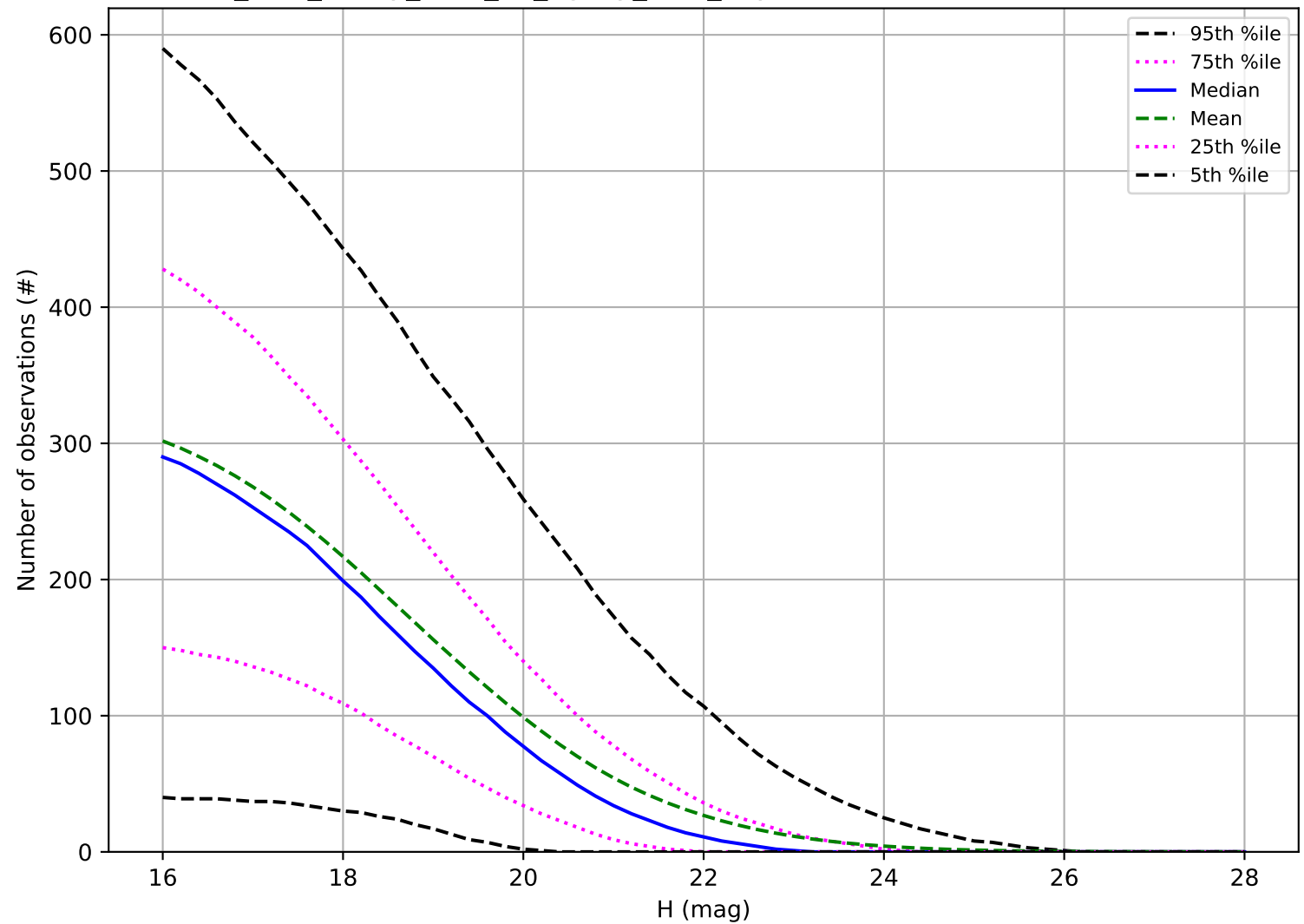
too_elab_heavy_r128_d2_ugrizy_v3.4_10yrs: Number of observations PHA
