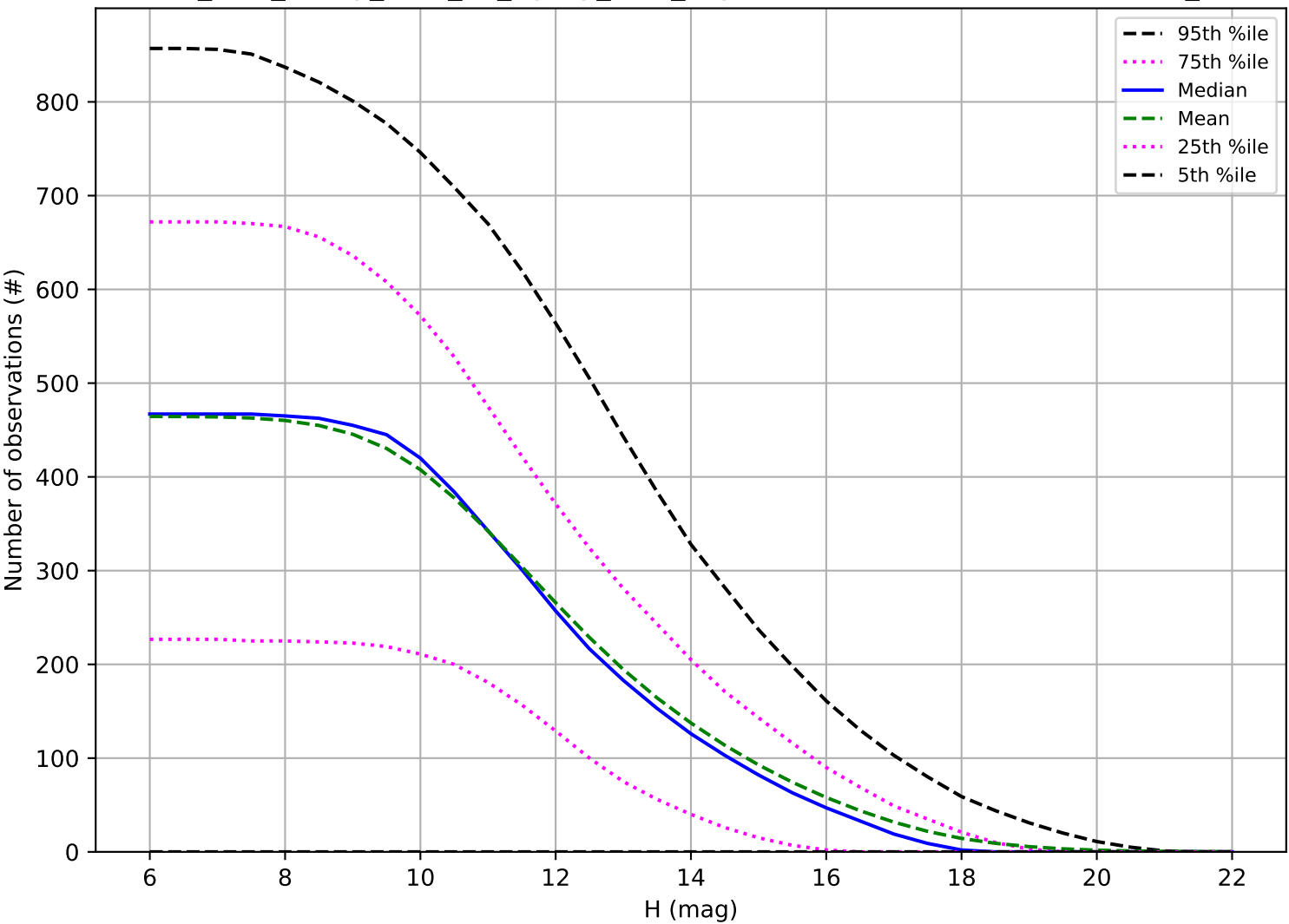
too_elab_heavy_r128_d2_ugrizy_v3.4_10yrs: Number of observations OCC_r5
