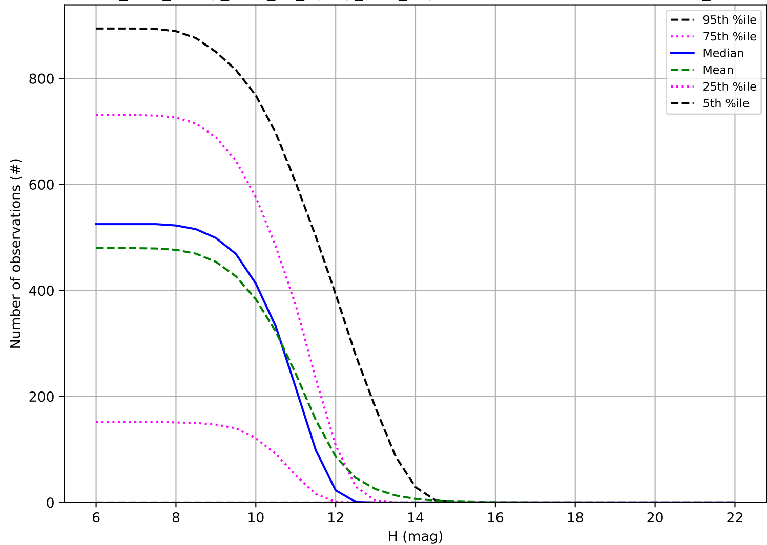
too_elab_heavy_r128_d2_ugrizy_v3.4_10yrs: Number of observations OCC_r20
