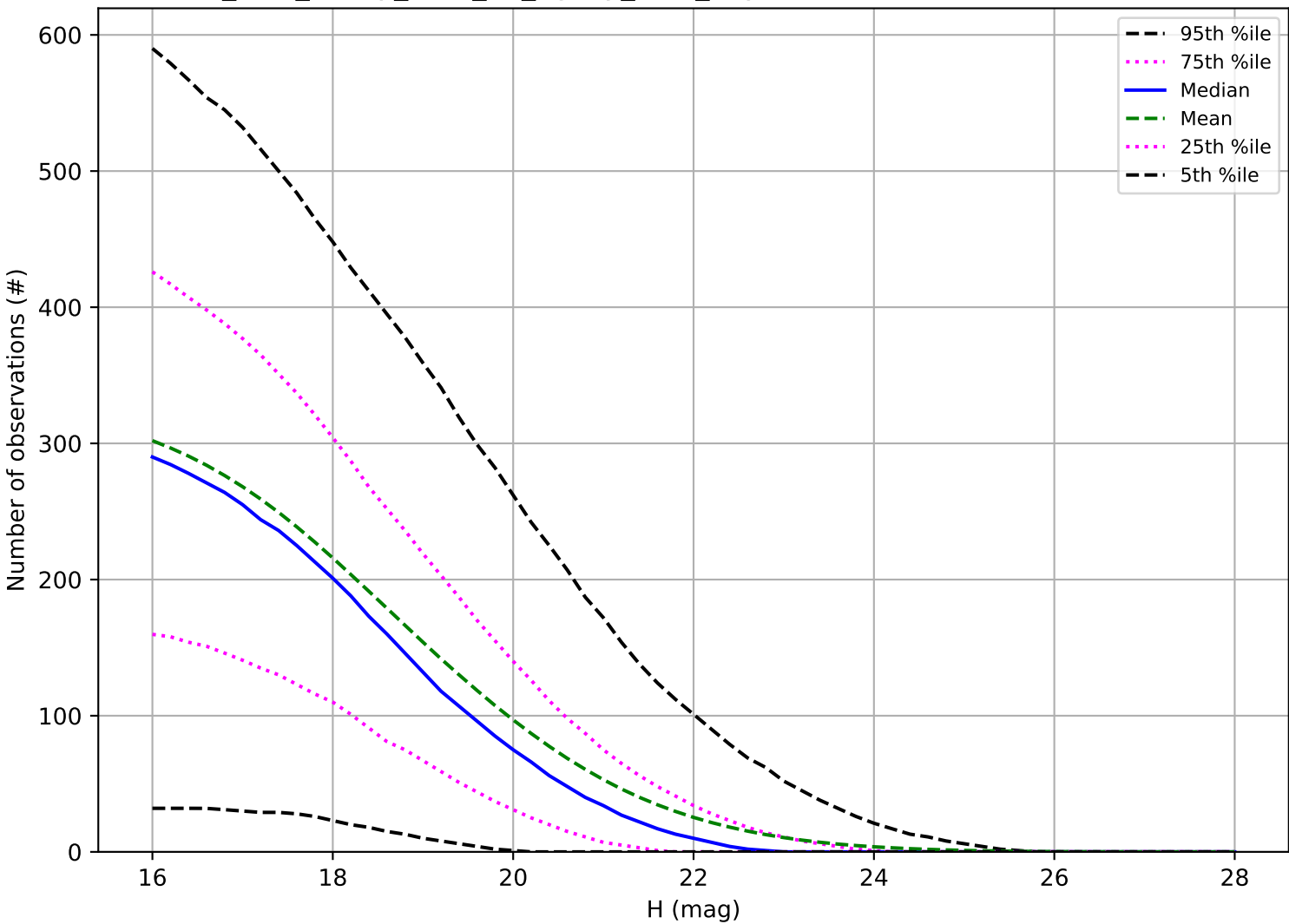
too_elab_heavy_r128_d2_ugrizy_v3.4_10yrs: Number of observations NEO
