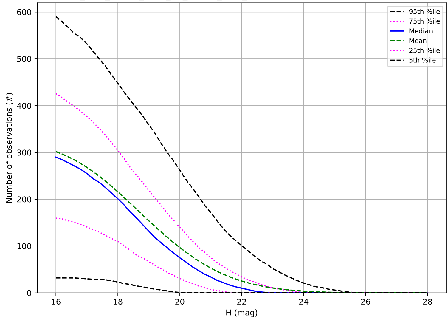
too_elab_heavy_r128_d2_ugrizy_v3.4_10yrs: Number of observations NEO
