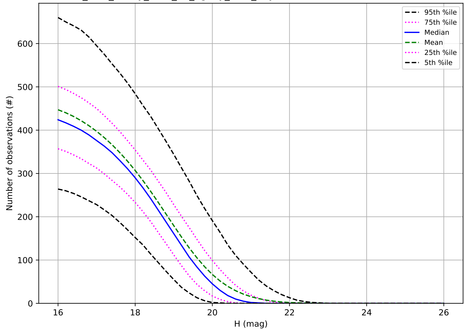
too_elab_heavy_r128_d2_ugrizy_v3.4_10yrs: Number of observations MBA
