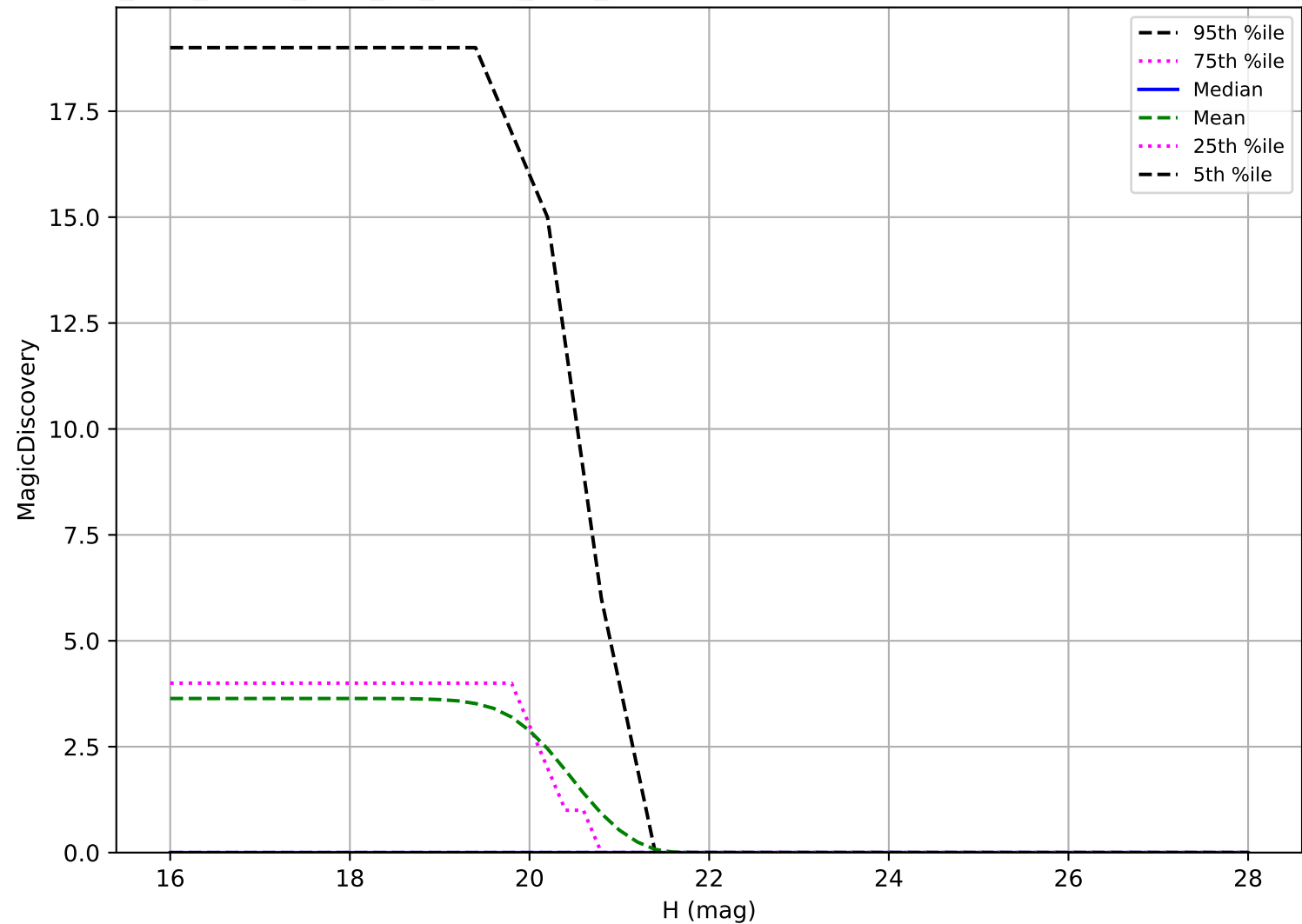
too_elab_heavy_r128_d2_ugrizy_v3.4_10yrs: Vatira 6 detections in 60 nights detection loss
