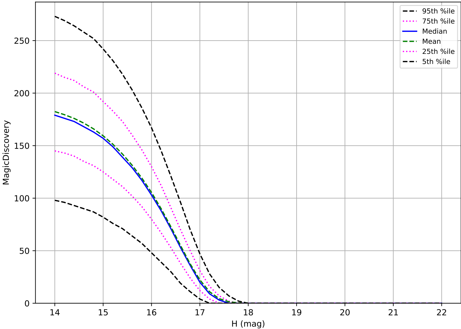
too_elab_heavy_r128_d2_ugrizy_v3.4_10yrs: Trojan 6 detections in 60 nights detection loss
