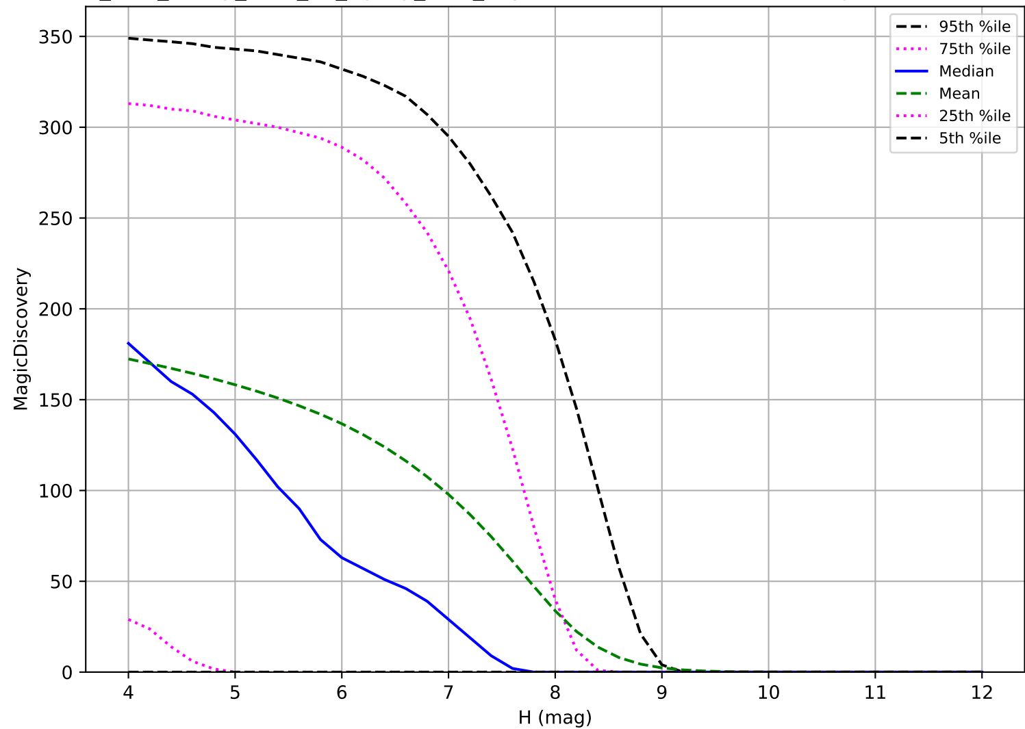
too_elab_heavy_r128_d2_ugrizy_v3.4_10yrs: TNO 6 detections in 60 nights detection loss
