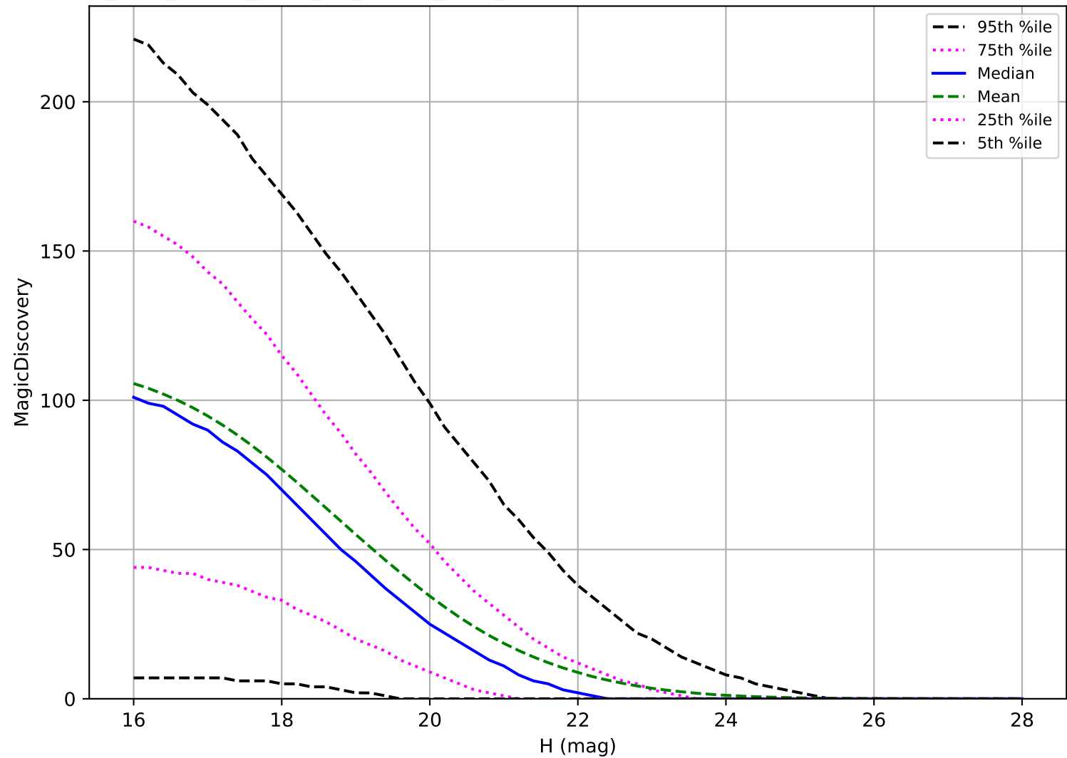
too_elab_heavy_r128_d2_ugrizy_v3.4_10yrs: PHA 6 detections in 60 nights detection loss
