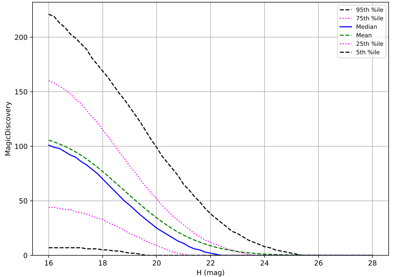
too_elab_heavy_r128_d2_ugrizy_v3.4_10yrs: PHA 6 detections in 60 nights detection loss
