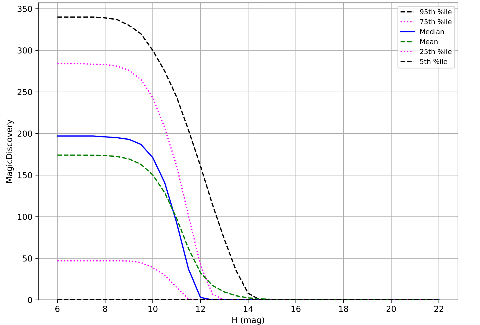
too_elab_heavy_r128_d2_ugrizy_v3.4_10yrs: OCC_r20 6 detections in 60 nights detection loss
