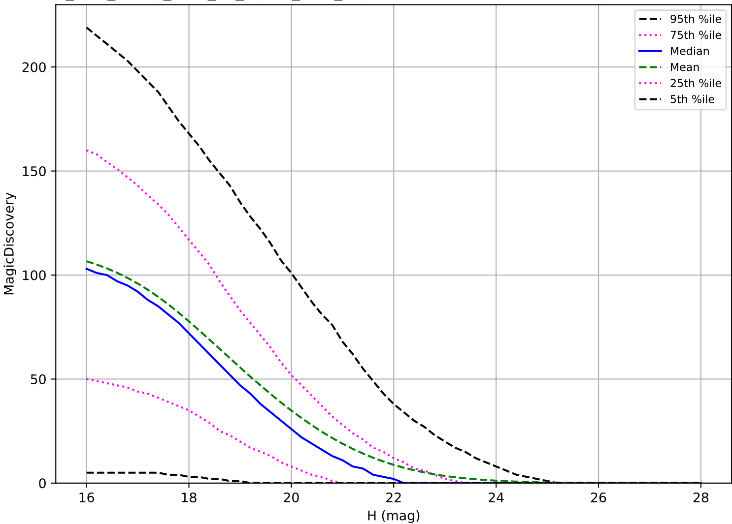
too_elab_heavy_r128_d2_ugrizy_v3.4_10yrs: NEO 6 detections in 60 nights detection loss
