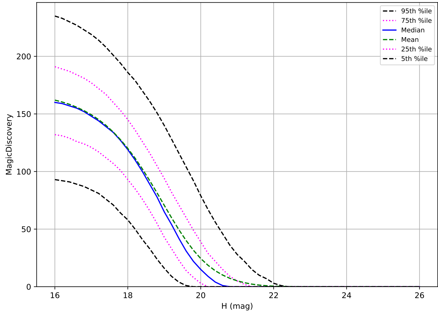
too_elab_heavy_r128_d2_ugrizy_v3.4_10yrs: MBA 6 detections in 60 nights detection loss
