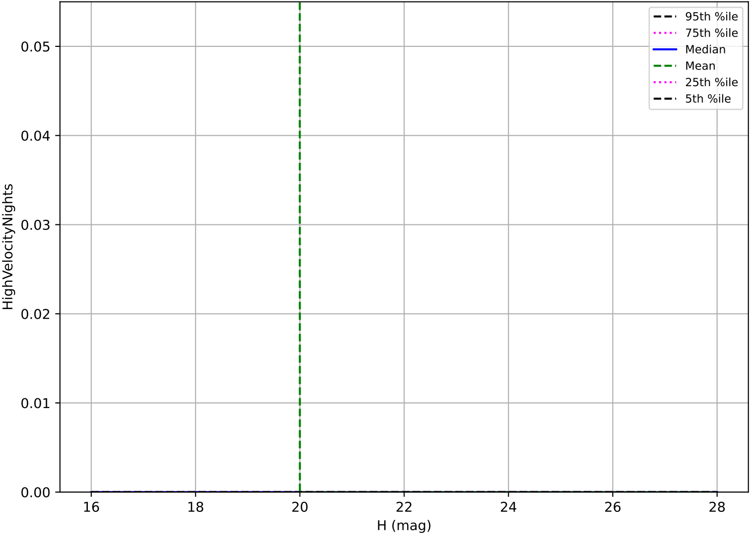
too_elab_heavy_r128_d2_ugrizy_v3.4_10yrs: Vatira High velocity pair detection loss
