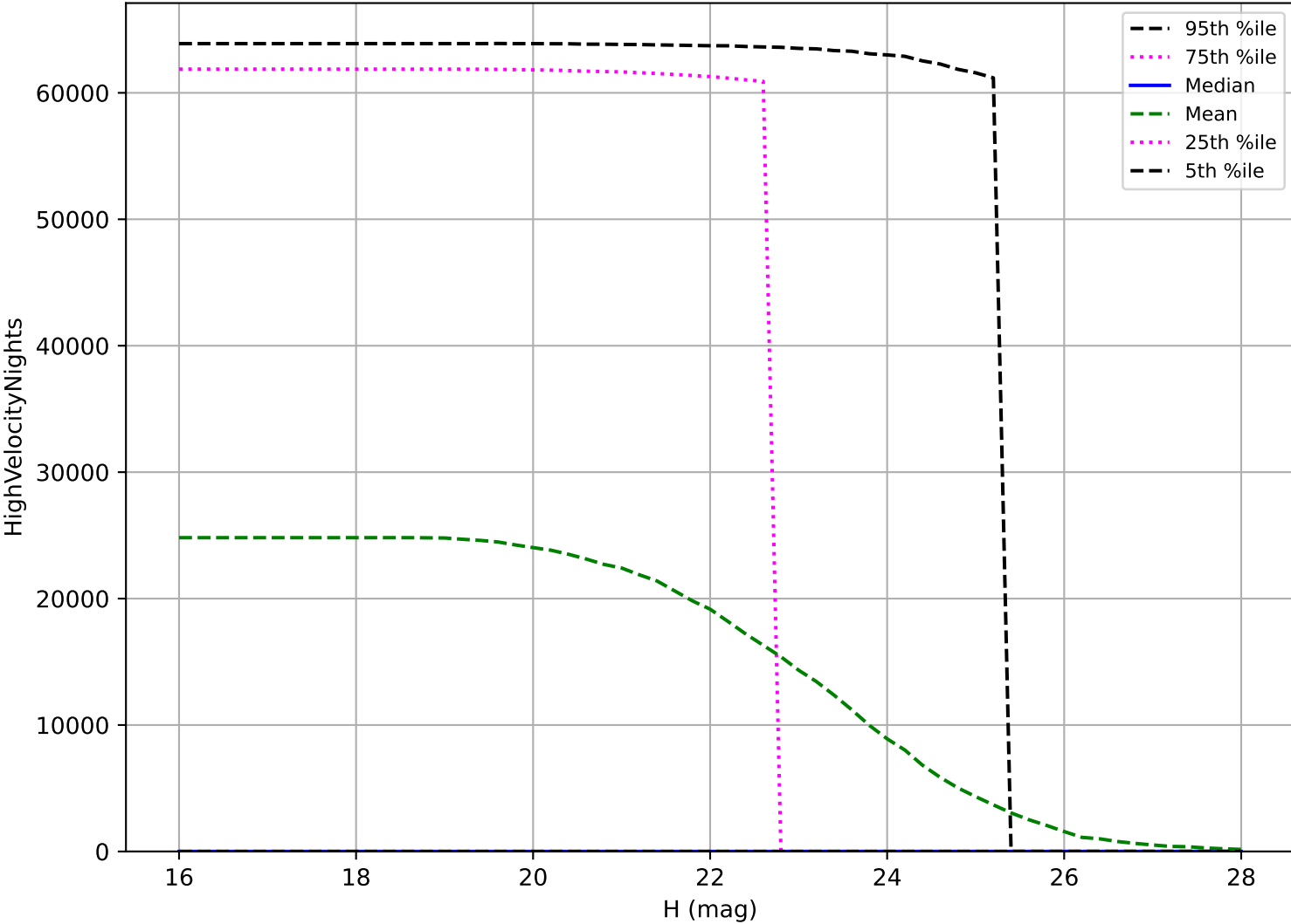
too_elab_heavy_r128_d2_ugrizy_v3.4_10yrs: PHA High velocity pair detection loss
