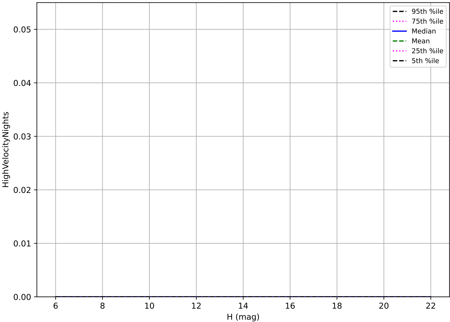
too_elab_heavy_r128_d2_ugrizy_v3.4_10yrs: OCC_r5 High velocity pair detection loss
