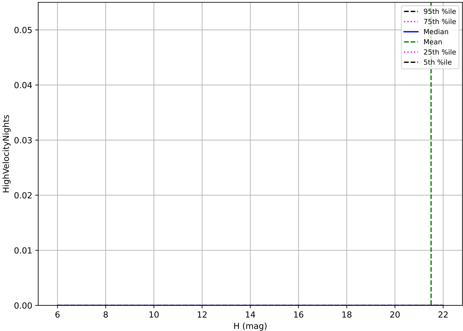
too_elab_heavy_r128_d2_ugrizy_v3.4_10yrs: OCC_r20 High velocity pair detection loss
