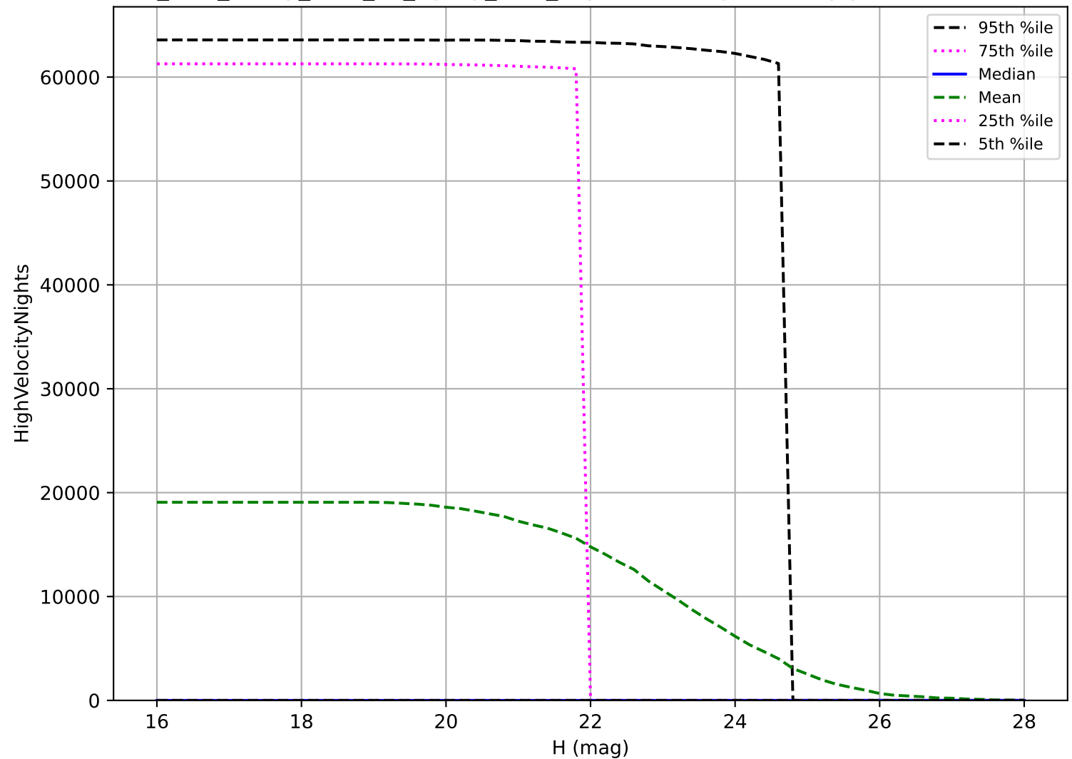
too_elab_heavy_r128_d2_ugrizy_v3.4_10yrs: NEO High velocity pair detection loss
