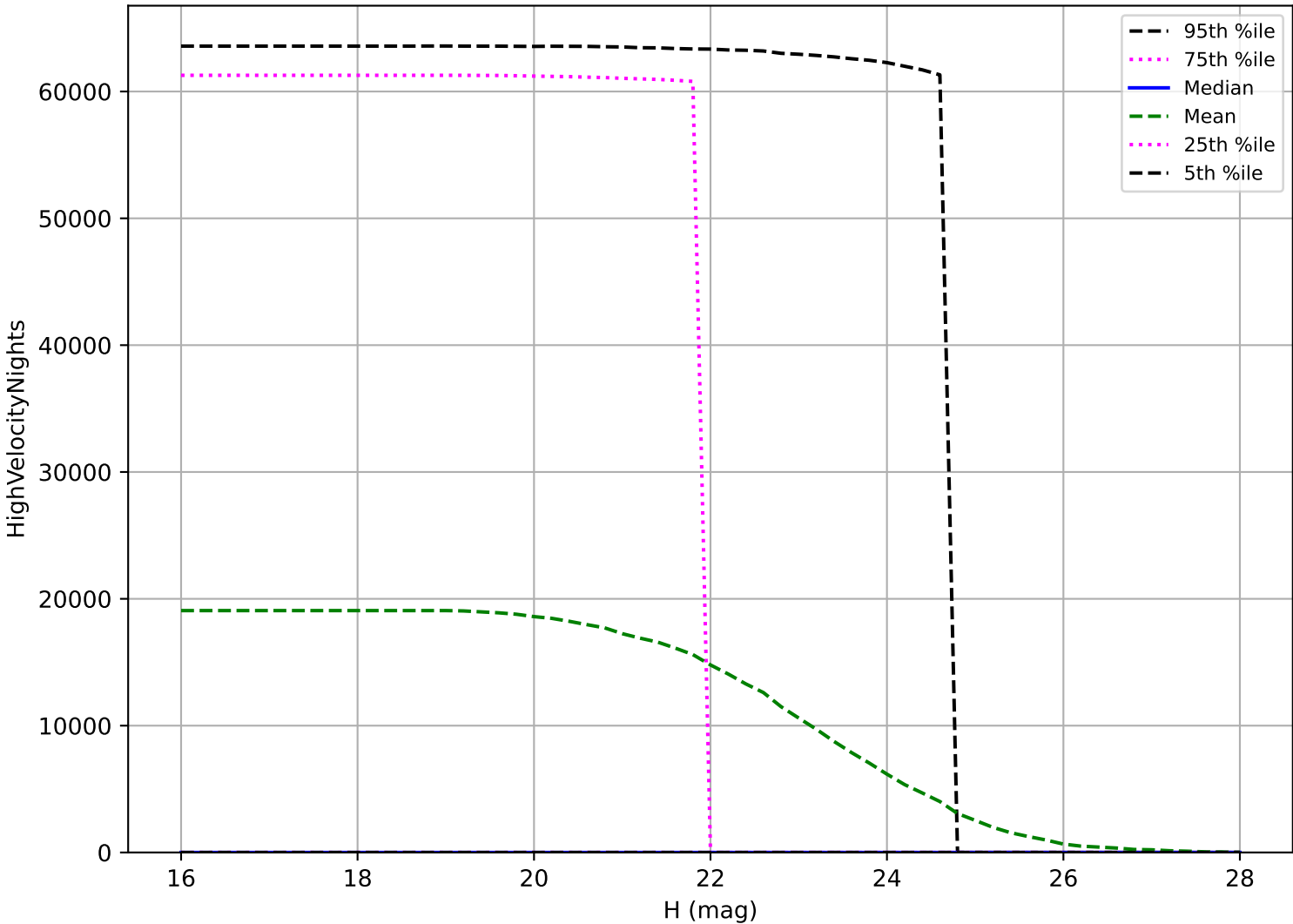
too_elab_heavy_r128_d2_ugrizy_v3.4_10yrs: NEO High velocity pair detection loss
