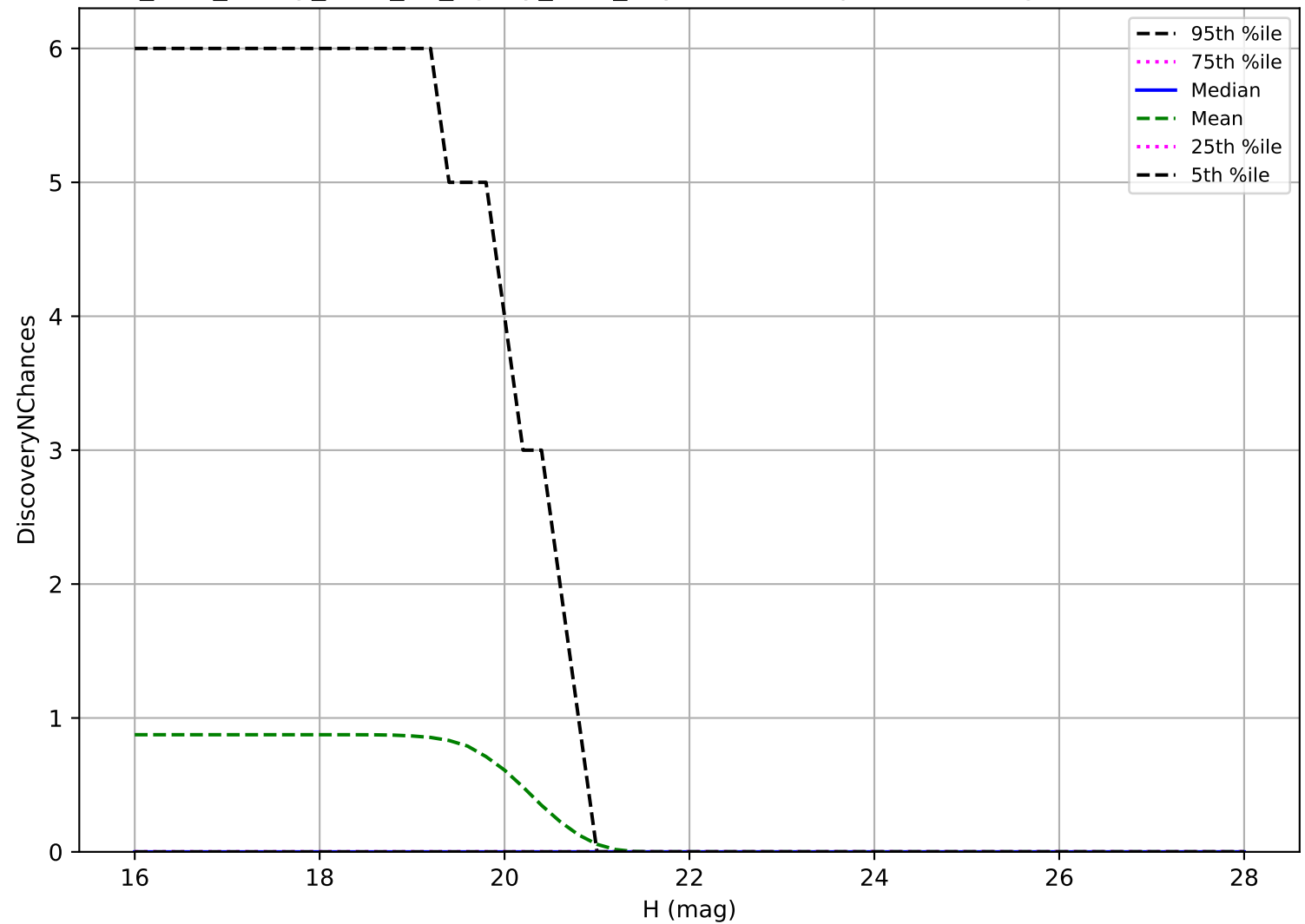
too_elab_heavy_r128_d2_ugrizy_v3.4_10yrs: Vatira 3 pairs in 15 nights detection loss
