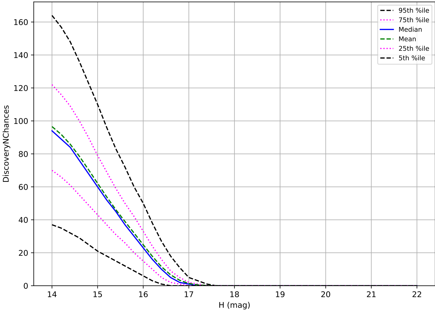
too_elab_heavy_r128_d2_ugrizy_v3.4_10yrs: Trojan 3 pairs in 15 nights detection loss
