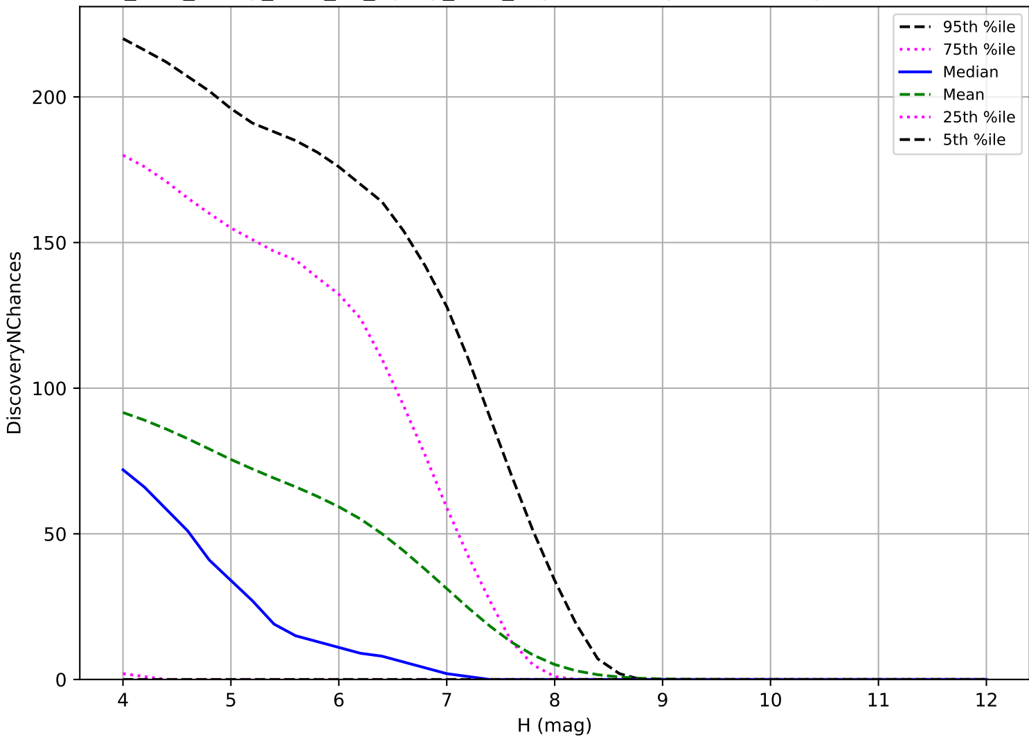
too_elab_heavy_r128_d2_ugrizy_v3.4_10yrs: TNO 3 pairs in 15 nights detection loss
