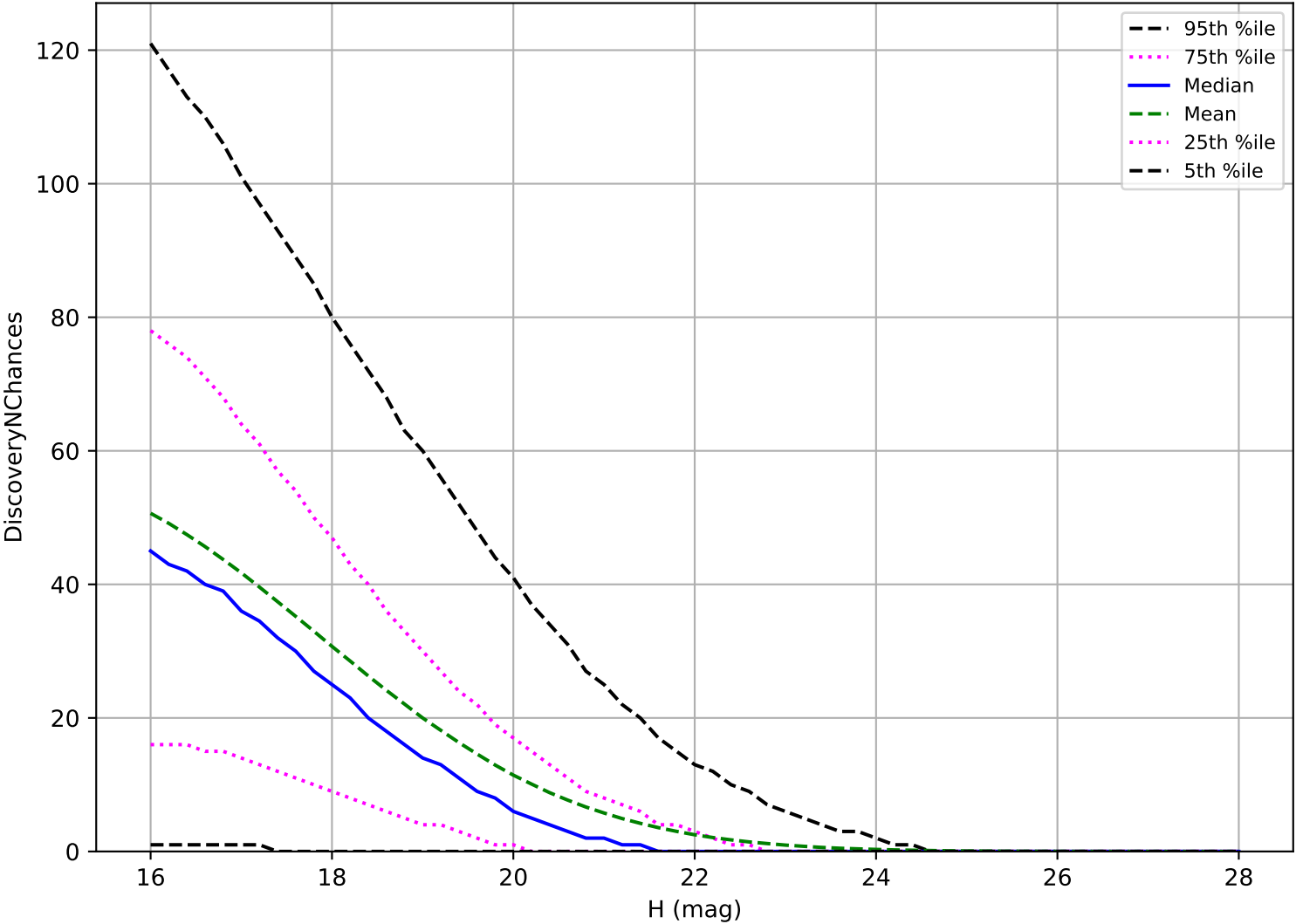
too_elab_heavy_r128_d2_ugrizy_v3.4_10yrs: PHA 3 pairs in 15 nights detection loss
