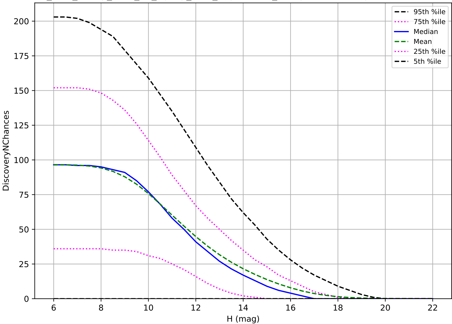
too_elab_heavy_r128_d2_ugrizy_v3.4_10yrs: OCC_r5 3 pairs in 15 nights detection loss
