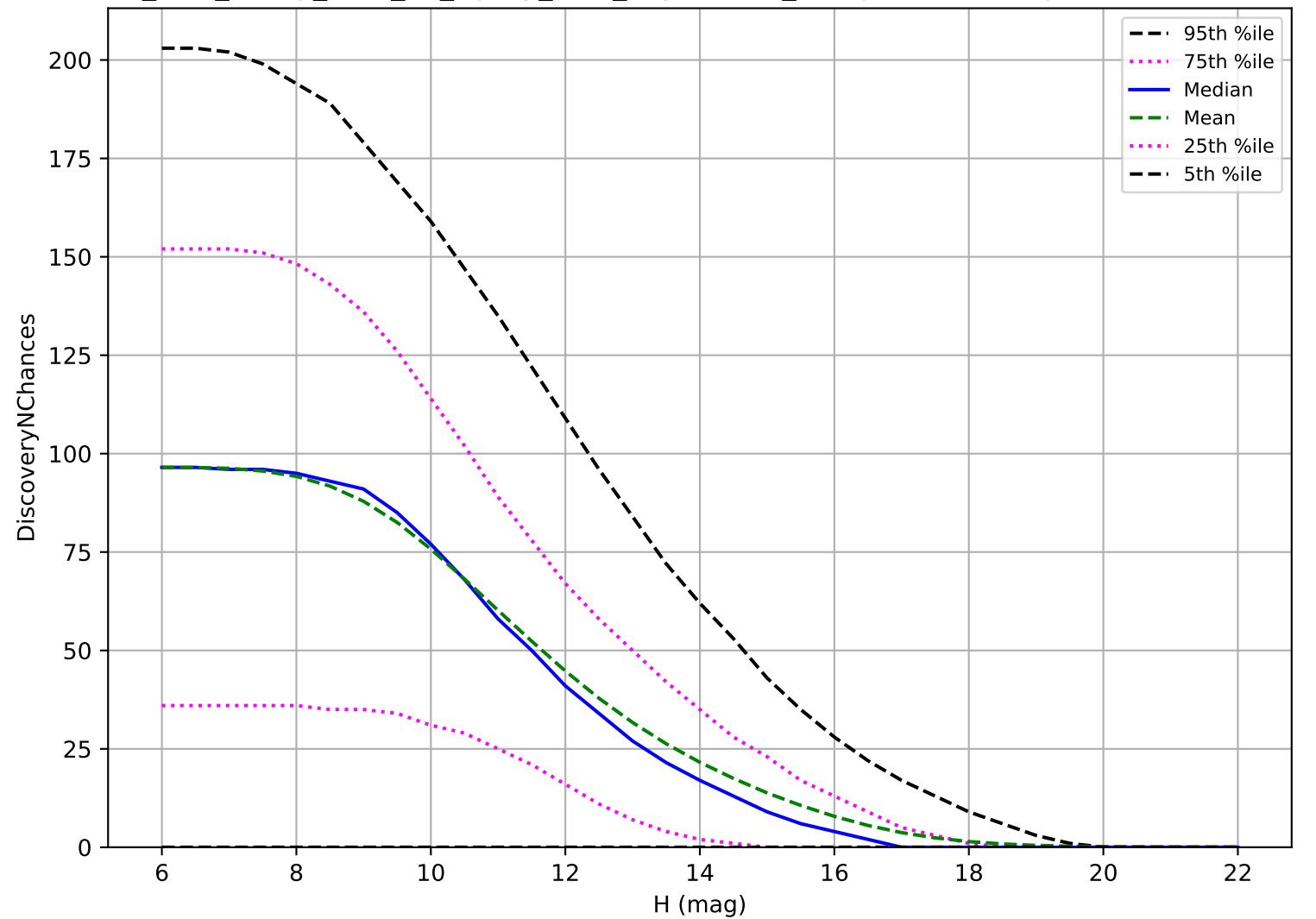
too_elab_heavy_r128_d2_ugrizy_v3.4_10yrs: OCC_r5 3 pairs in 15 nights detection loss
