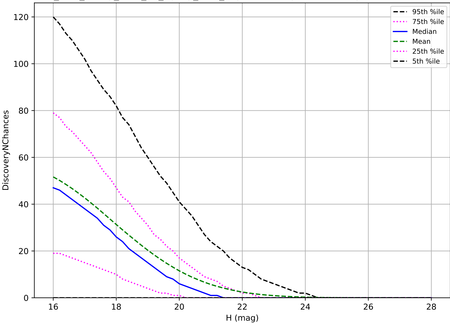
too_elab_heavy_r128_d2_ugrizy_v3.4_10yrs: NEO 3 pairs in 15 nights detection loss
