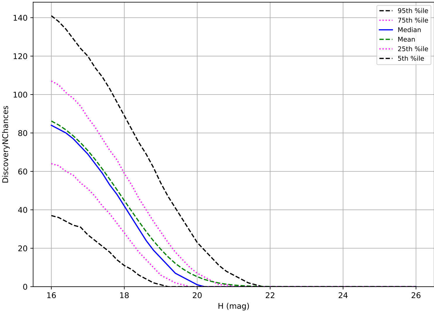
too_elab_heavy_r128_d2_ugrizy_v3.4_10yrs: MBA 3 pairs in 15 nights detection loss
