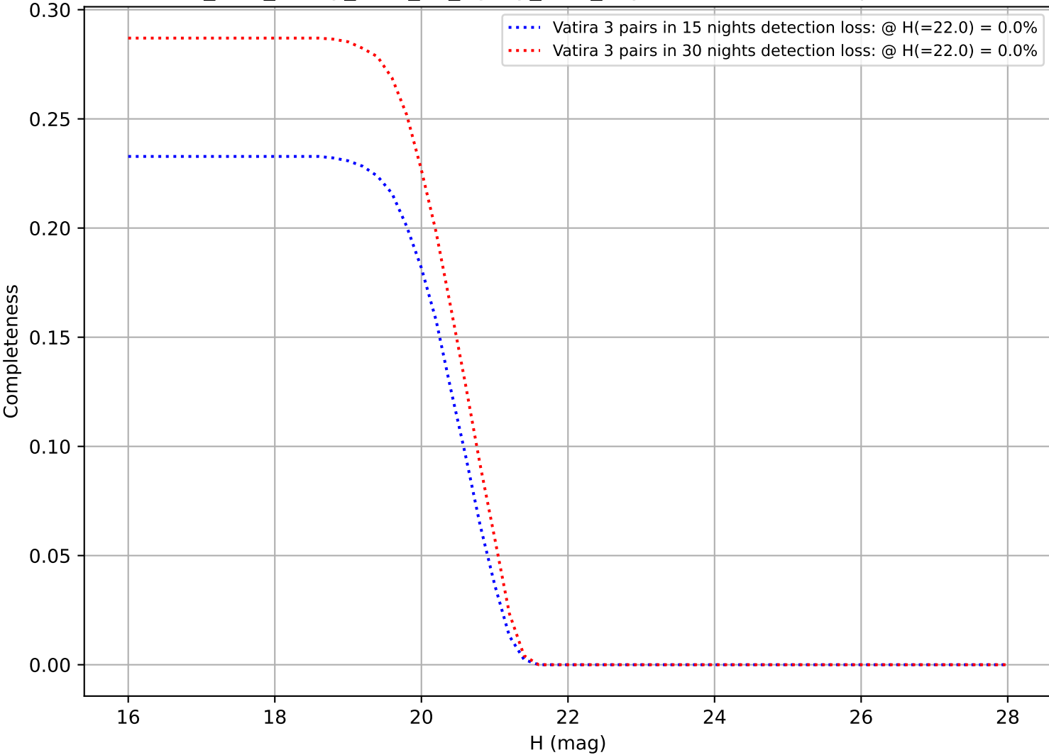
too_elab_heavy_r128_d2_ugrizy_v3.4_10yrs: DifferentialCompleteness
