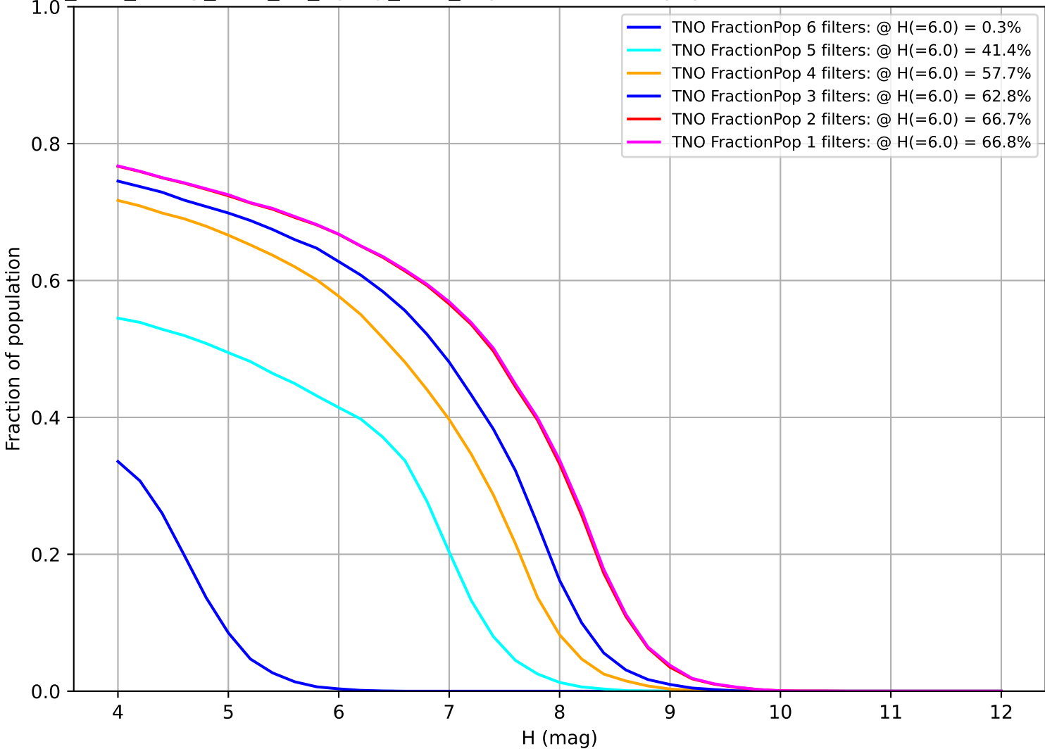
too_elab_heavy_r128_d2_ugrizy_v3.4_10yrs: Fraction of population with colors in X filters TNO
