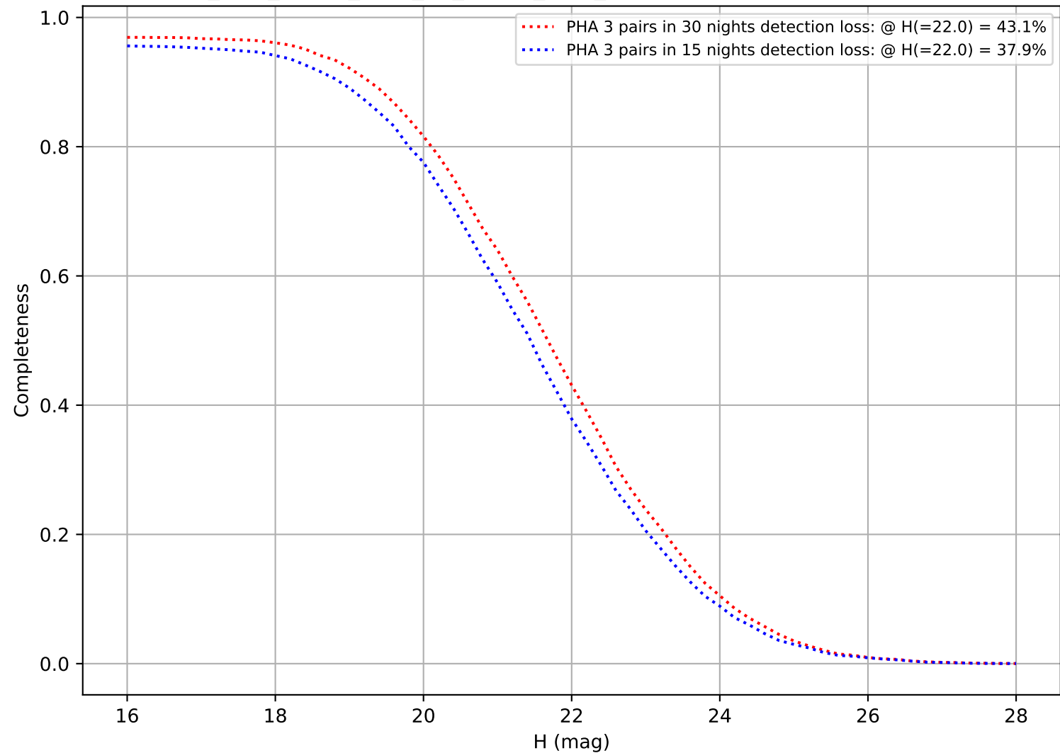
too_elab_heavy_r128_d2_ugrizy_v3.4_10yrs: DifferentialCompleteness
