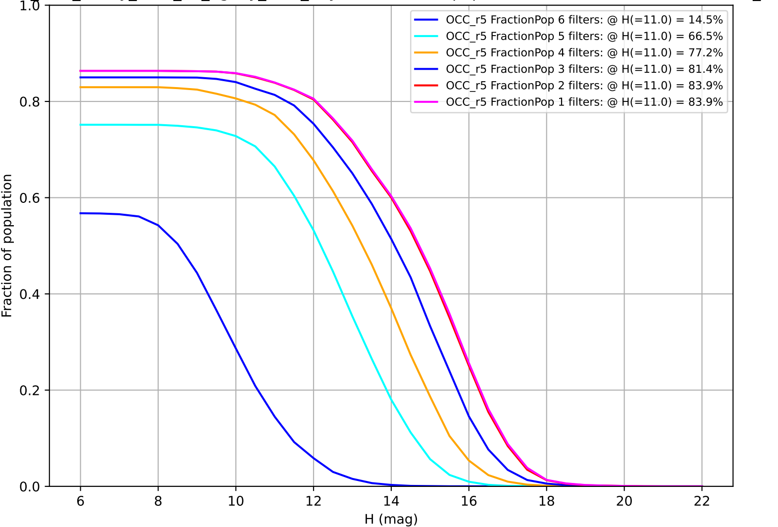
too_elab_heavy_r128_d2_ugrizy_v3.4_10yrs: Fraction of population with colors in X filters OCC_r5
