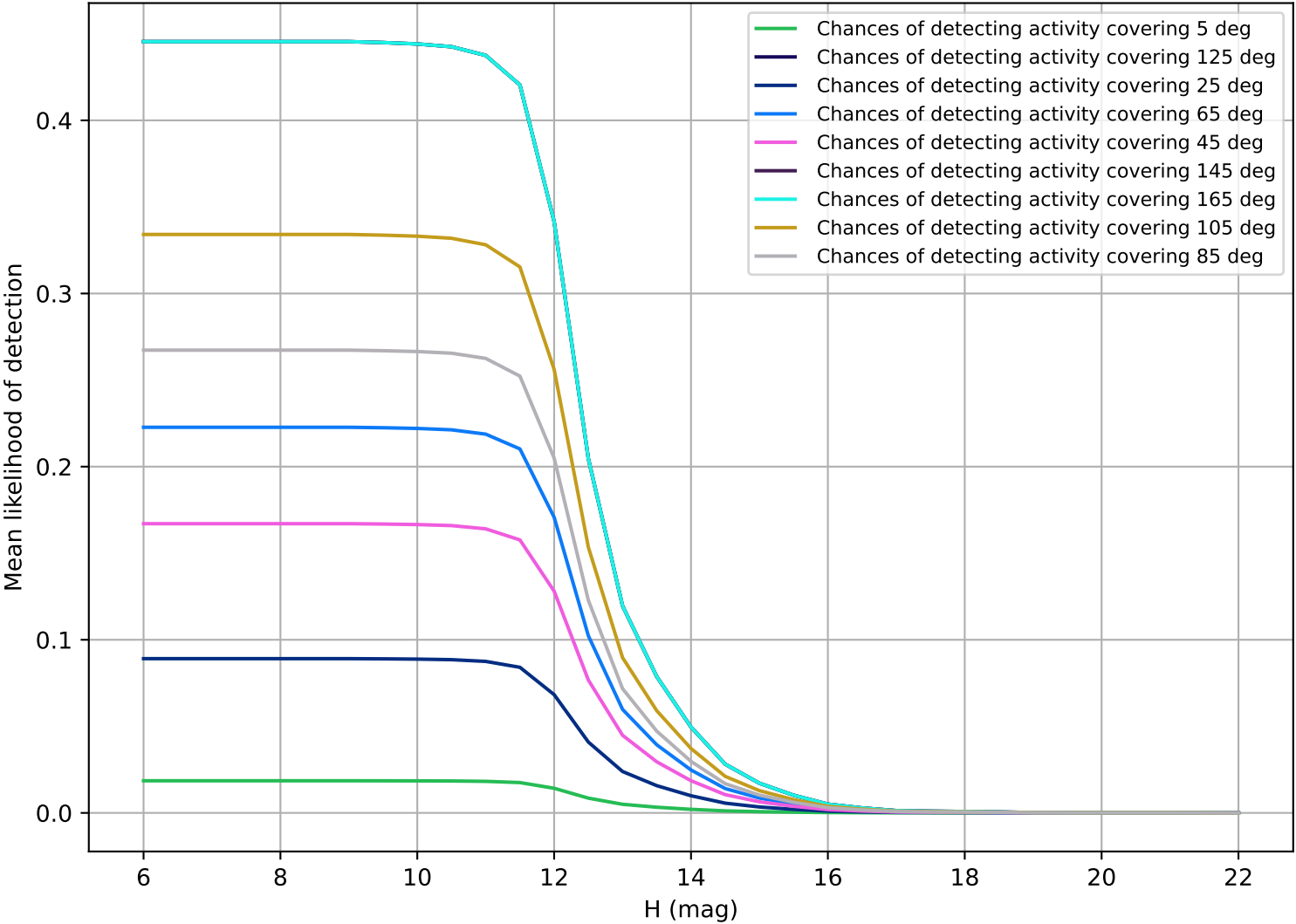
too_elab_heavy_r128_d2_ugrizy_v3.4_10yrs OCC_r20
