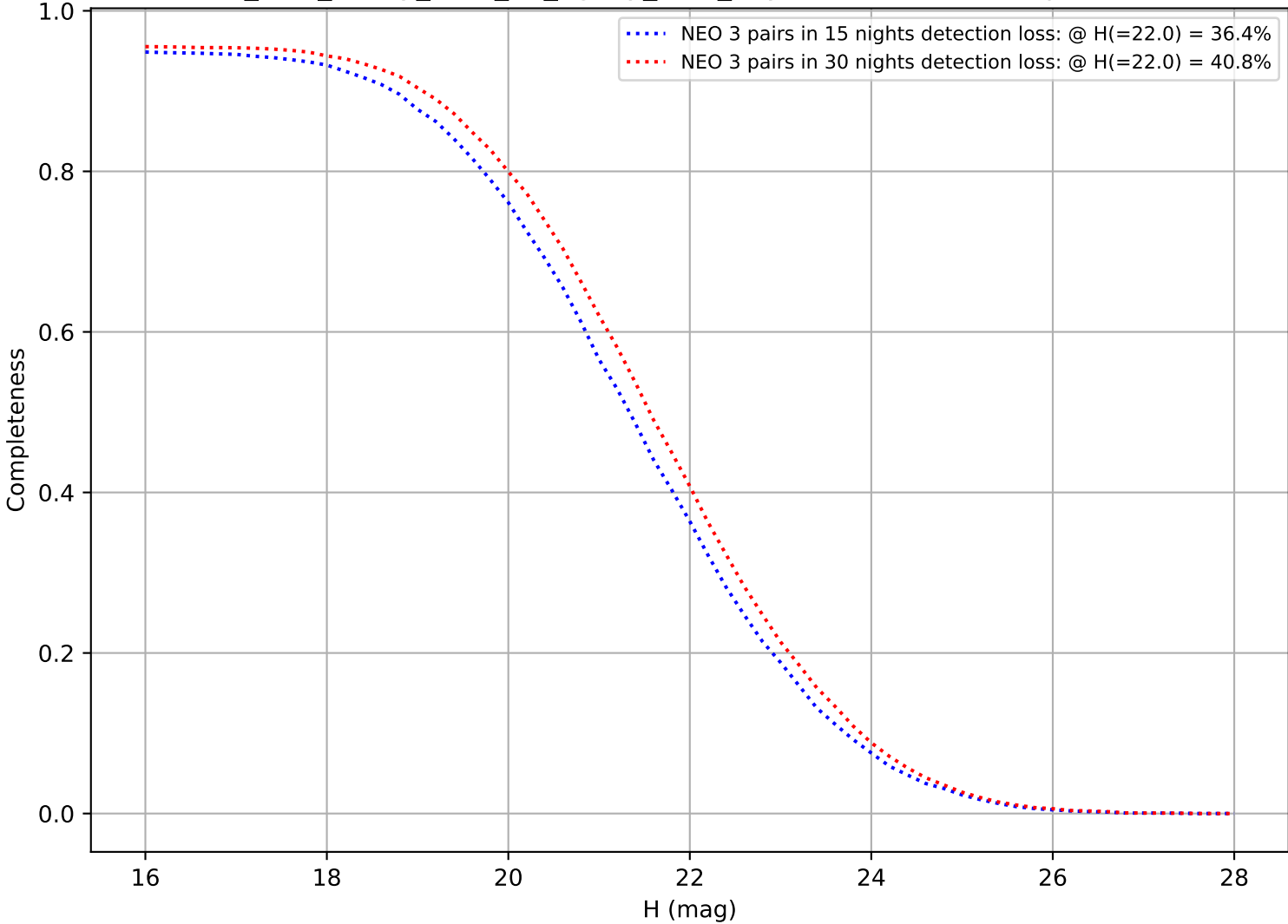
too_elab_heavy_r128_d2_ugrizy_v3.4_10yrs: DifferentialCompleteness
