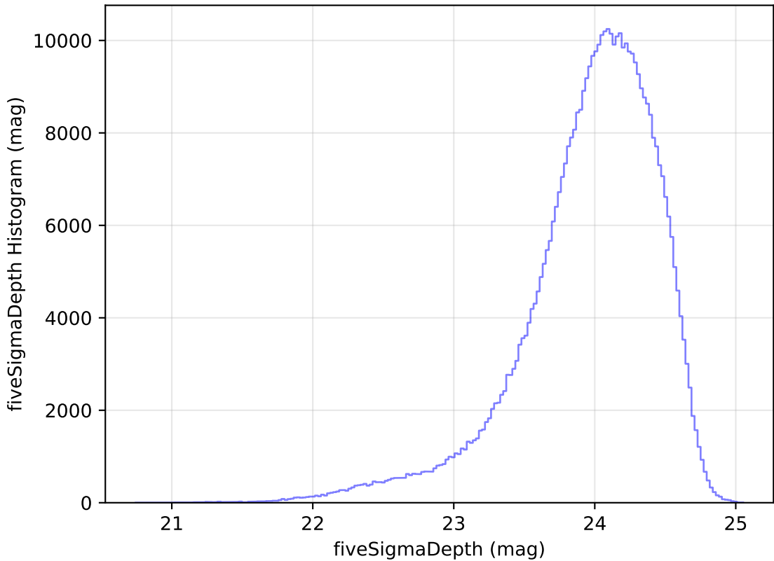
too_elab_heavy_r128_d2_ugrizy_v3.4_10yrs r: fiveSigmaDepth Histogram
