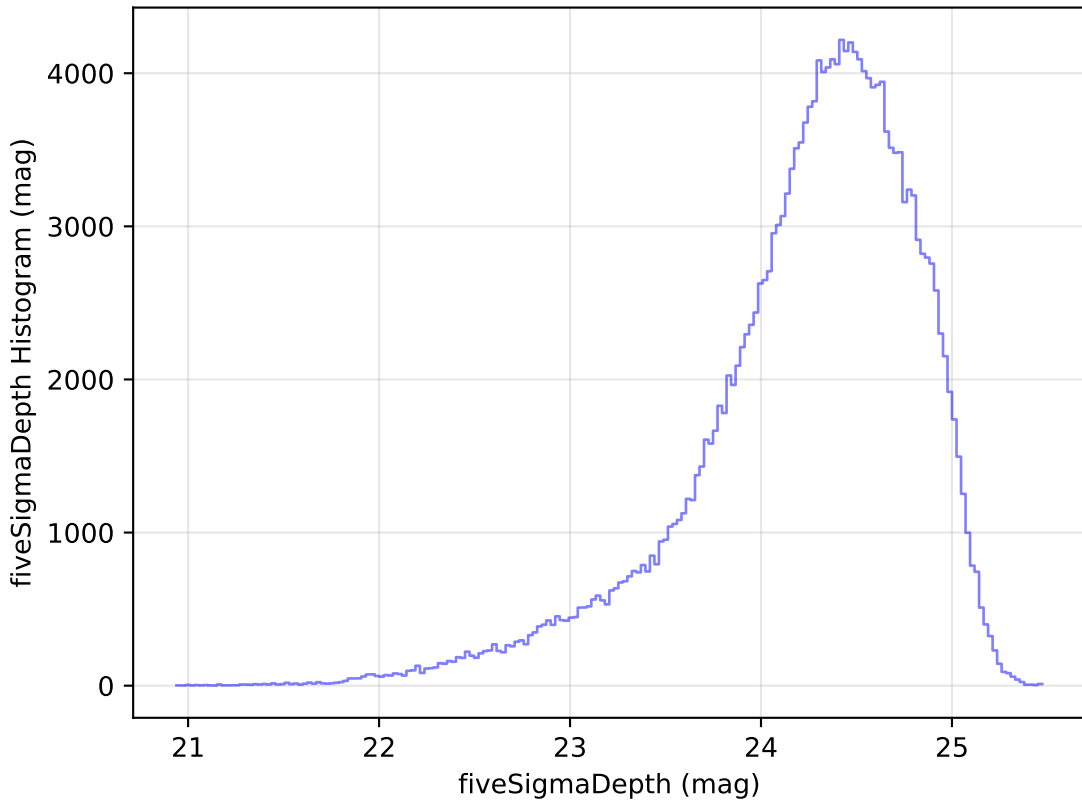
too_elab_heavy_r128_d2_ugrizy_v3.4_10yrs g: fiveSigmaDepth Histogram
