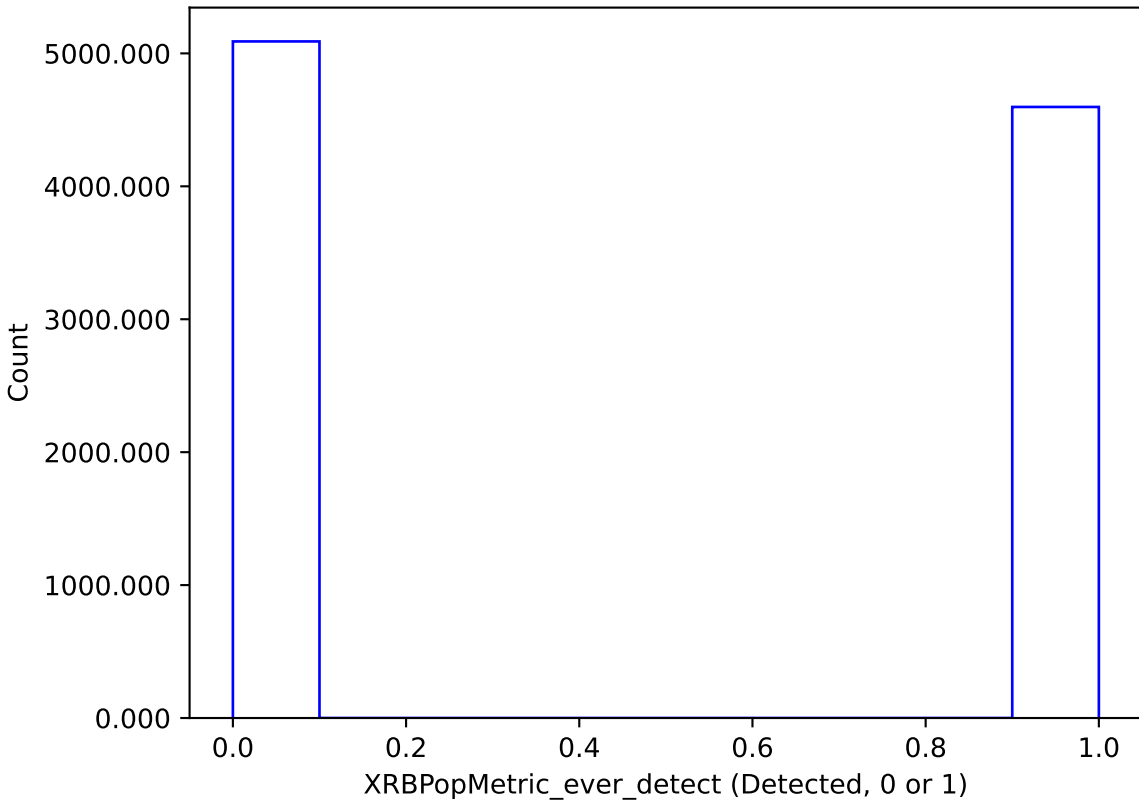
too_elab_heavy_r128_d2_ugrizy_v3.4_10yrs : XRBPoMetric_ever_detect
