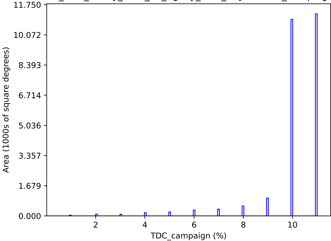
too_elab_heavy_r128_d2_ugrizy_v3.4_10yrs : TDC_campaign
