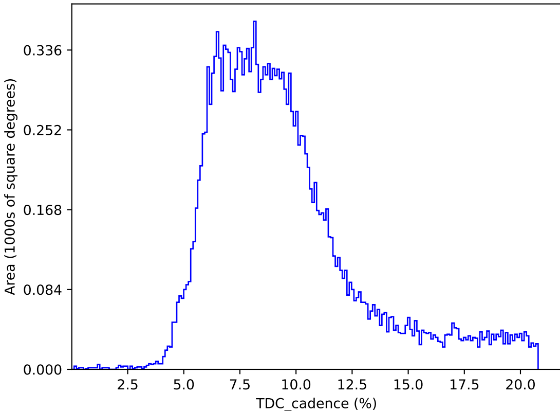
too_elab_heavy_r128_d2_ugrizy_v3.4_10yrs : TDC_cadence
