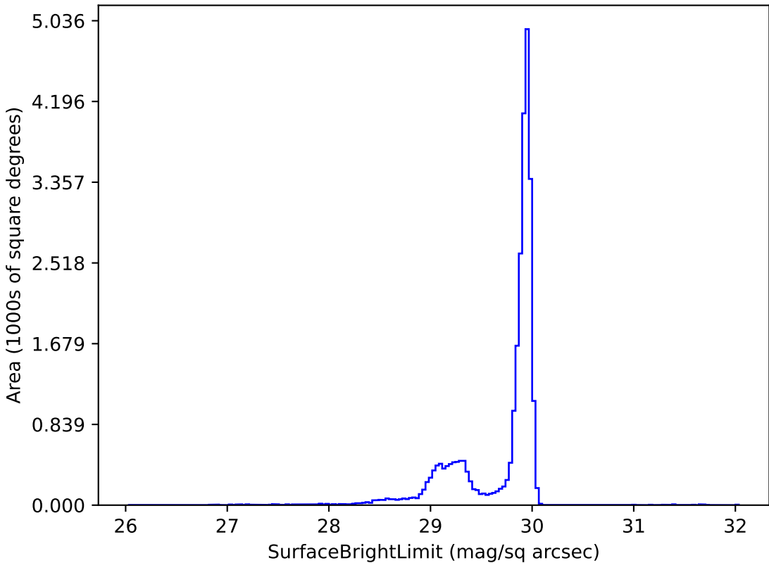
too_elab_heavy_r128_d2_ugrizy_v3.4_10yrs i: SurfaceBrightLimit
