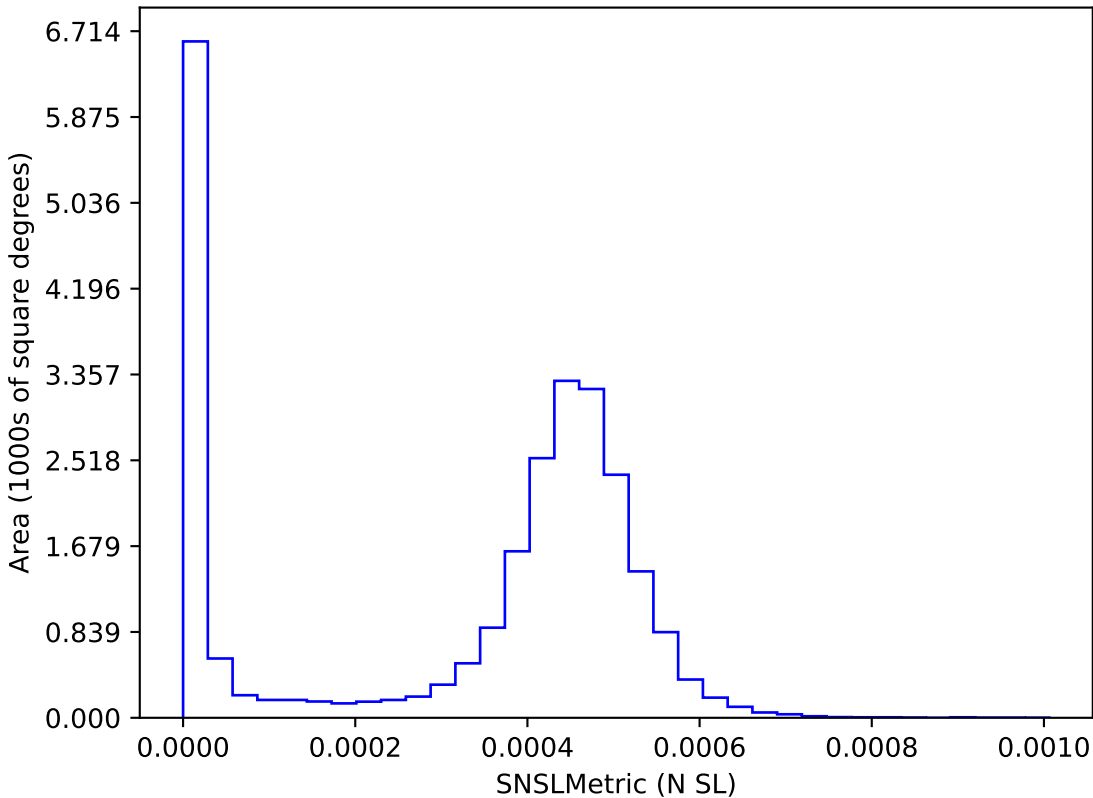
too_elab_heavy_r128_d2_ugrizy_v3.4_10yrs : SNSLMetric
