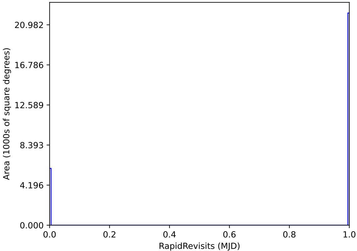
too_elab_heavy_r128_d2_ugrizy_v3.4_10yrs : RapidRevisits
